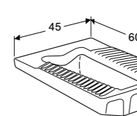
HURKTOILET Hurktoilet
